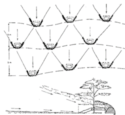
Figure 1. Pit Design
